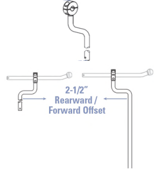
ONYX REARWARD OFF-SET VERTICAL ROD
