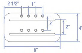
SLIDE MOUNT
